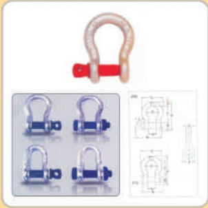
Forged Shackles
